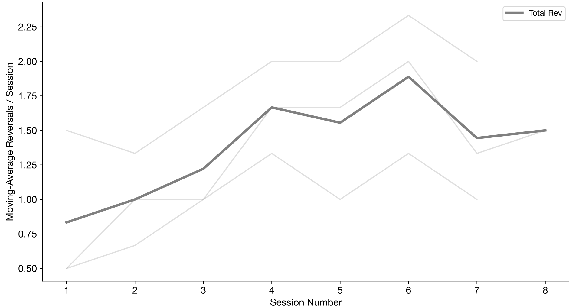
Moving-Average Total Reversals Over Time (n=3 subjects; sessions per subject=7–8; window=3)
